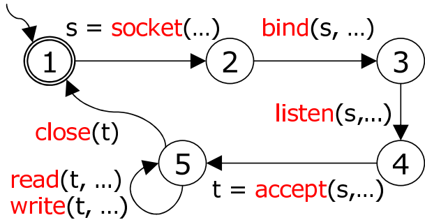
Figure 1. A simplified socket safety policy.
